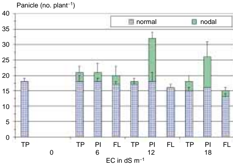
Figure 6. Effects of salinity stress on panicle numbers (IR64 phytroton experiment 1999).
